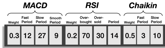
Figure 1: An example of an encoded candidate solution with three components.
