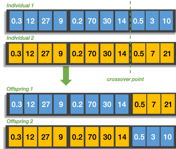
Figure 2: An example of a crossover operation.
