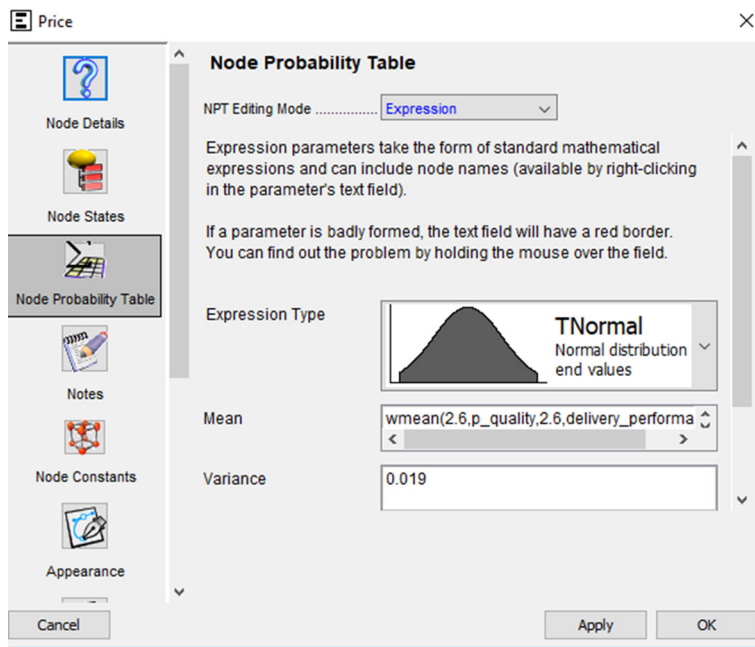
Fig. 8 Ranked nodes
