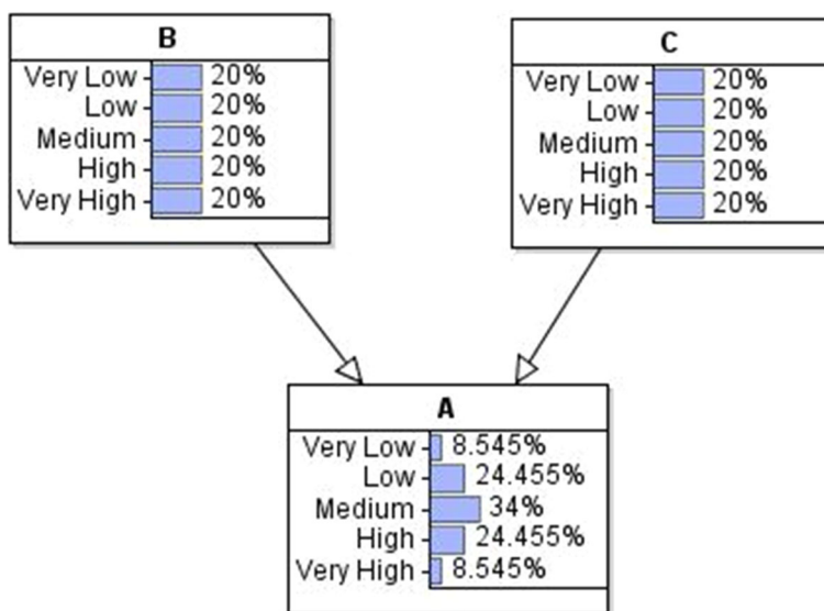
Fig. 3 Example network
