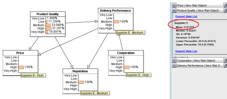
Fig. 10 Estimation of probability of product quality for supplier E
