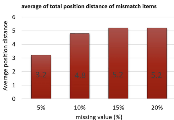
Fig. 12 Effect of average position on % of missing values
