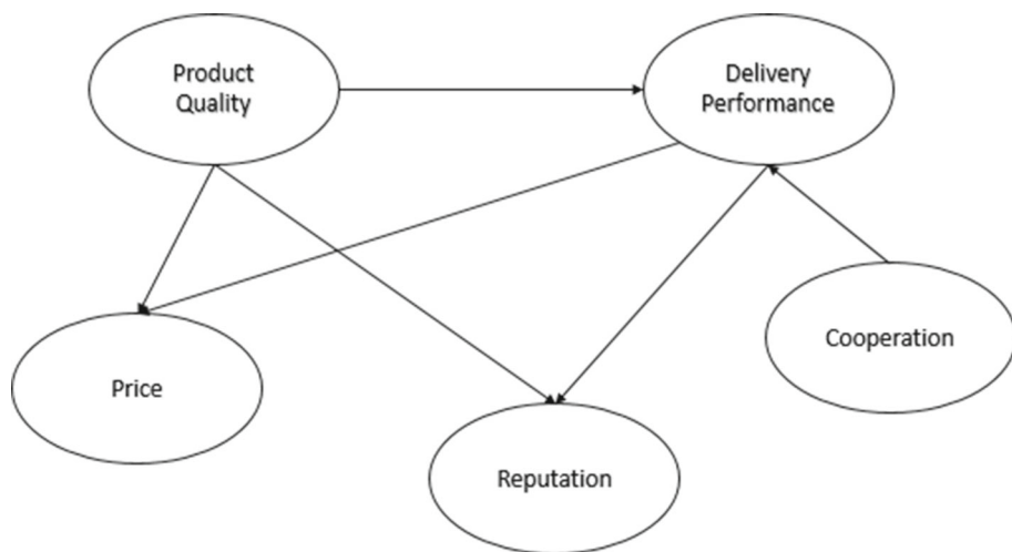
Fig. 7 Causal graph
